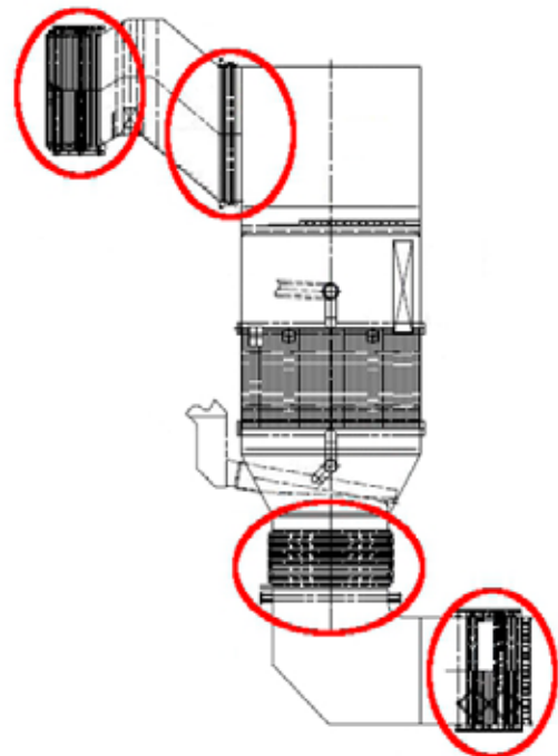
Installation position of the 4 large expansion joints
